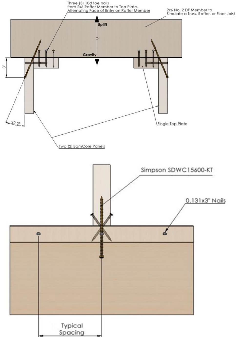
Figure 12. Top Plate of BamCore Prime Wall System and Truss/Rafter/Joist
