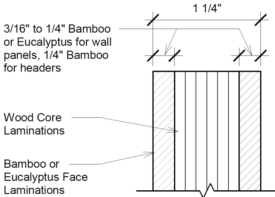
Figure 2. BamCore Prime Panel Construction
