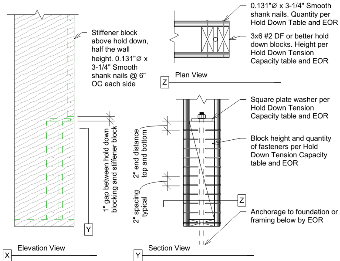
Figure 9. BamCore Hold Down for DuoShear Assemblies
