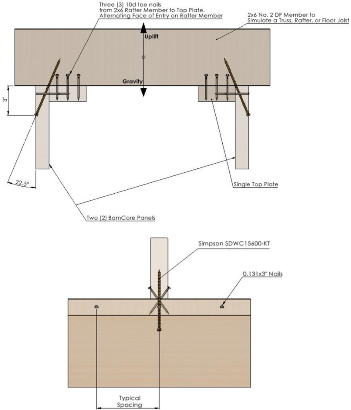
Figure 8. Top Plate of BamCore Prime Wall System and Truss/Rafter/Joist
