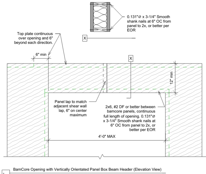
Figure 11. BamCore Opening with Vertically Orientated Panel Box Beam Header
