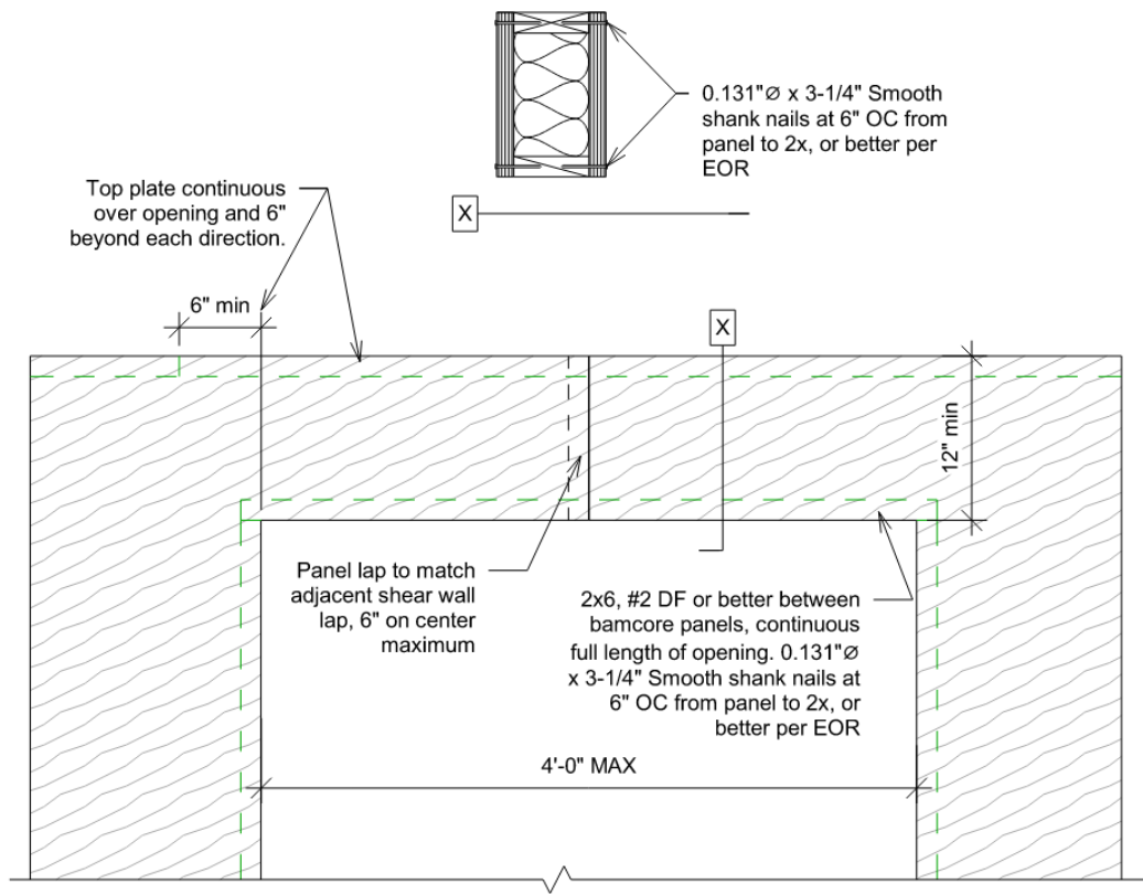
X BamCore Opening with Vertically Orientated Panel Box Beam Header (Elevation View)
