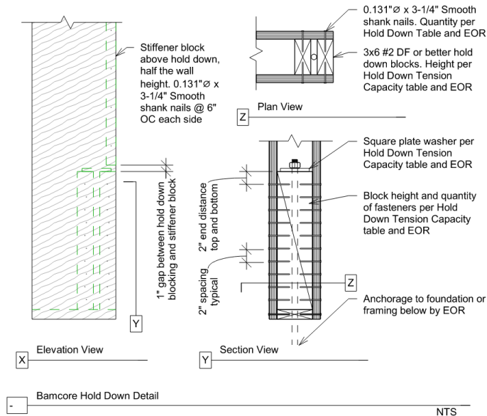
Figure 7. BamCore® Hold Down
