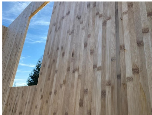
Figure 1. House Under Construction Using BamCore® Panelized Prime Wall™ System
