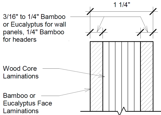
Figure 2. BamCore® Prime Panel Construction
